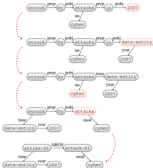
Figure 1: Example parse from dependency tree to AMR of the sentence fragment “...struck by cyber attacks in 2007.”
