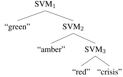
Figure 1: SVM classification
